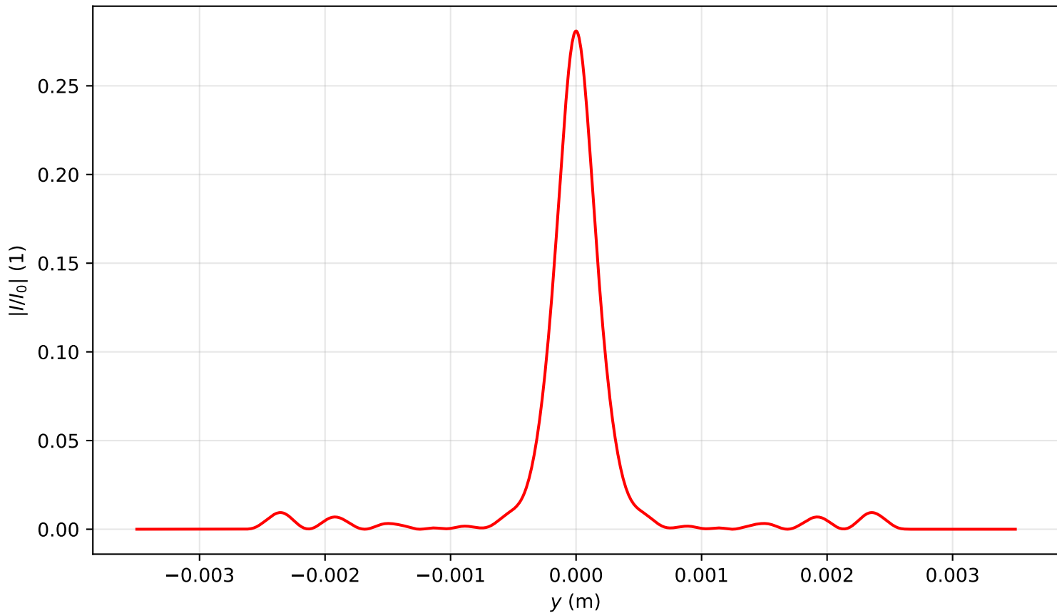
Intensity profile I(x = 0, y, z = 2.866)/I_0 , P_{in}=8.0P_{cr} , artificial time
